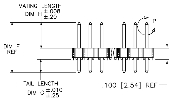
SINGLE ROW SIDE VIEW
