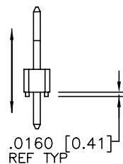
SINGLE ROW END VIEW
