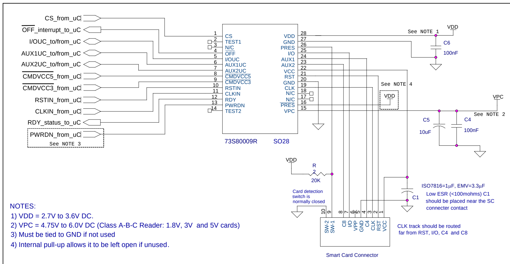
Figure 4: Typical 73S8009R Application Schematic
