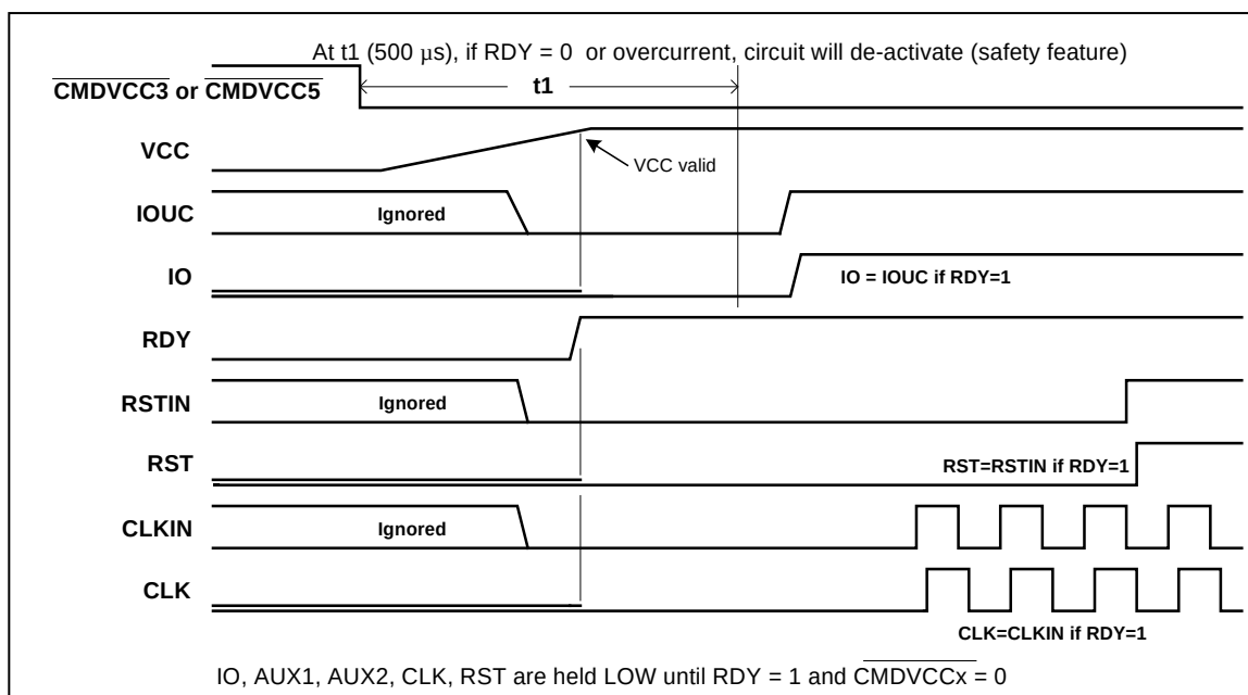
Figure 5: Activation Sequence
