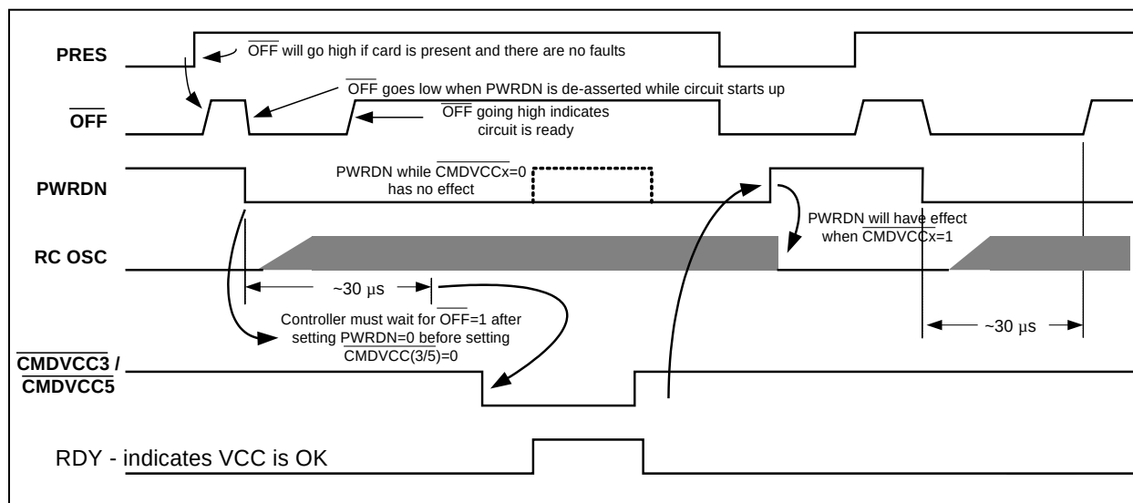
Figure 8: Power-down Operation
