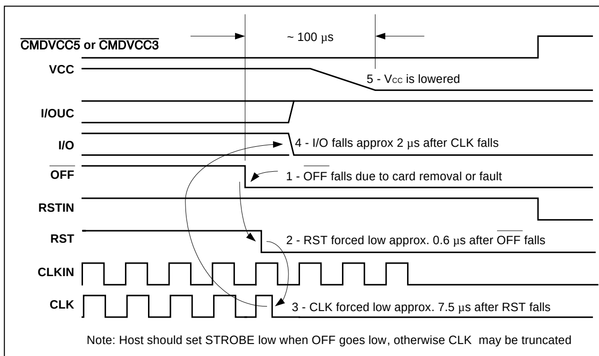
Figure 6: Deactivation Sequence
