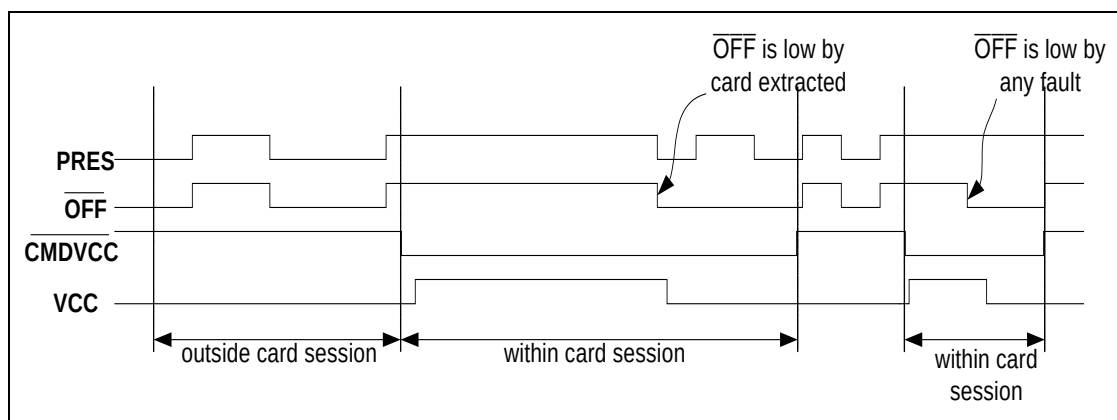
Figure 7: \overline{\text{OFF}} Activity Outside and Inside a Card Session
