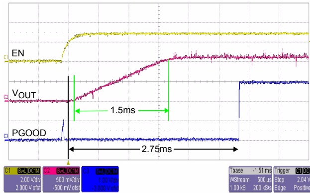
FIGURE 1. SOFT-START SEQUENCE
