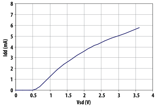
Figure 7. I_{dd} vs V_{sd} for V_{dd} = 1.8V , R_{bias} = 3.9k \Omega
