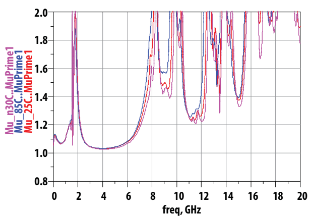
Figure 23. Edwards-Sinsky Input Stability Factor (Mu') at Vdd = 1.8V
