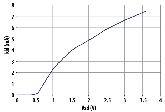
Figure 6. I_{dd} vs V_{sd} for V_{dd} = 2.7V , R_{bias} = 3.9k \Omega
