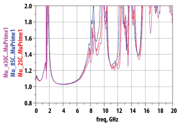
Figure 21. Edwards-Sinsky Input Stability Factor (Mu') at Vdd = 2.7V
