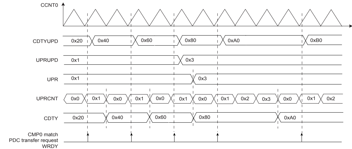
Figure 37-13. Method 3 (UPDM=2 and PTRM=1 and PTRCS=0)
