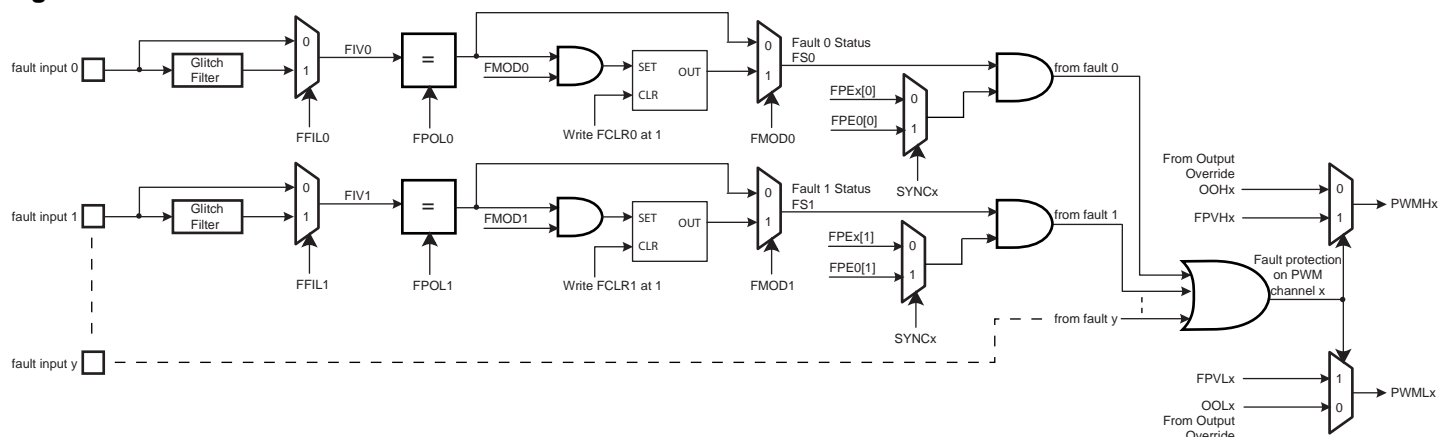
Figure 37-9. Fault Protection
