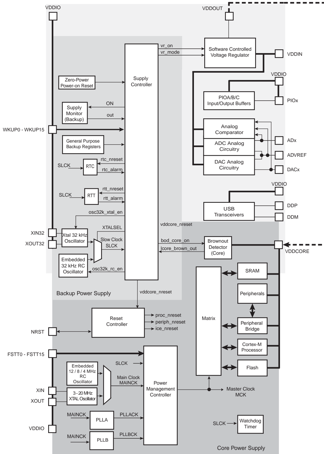
Figure 17-1. Supply Controller Block Diagram
