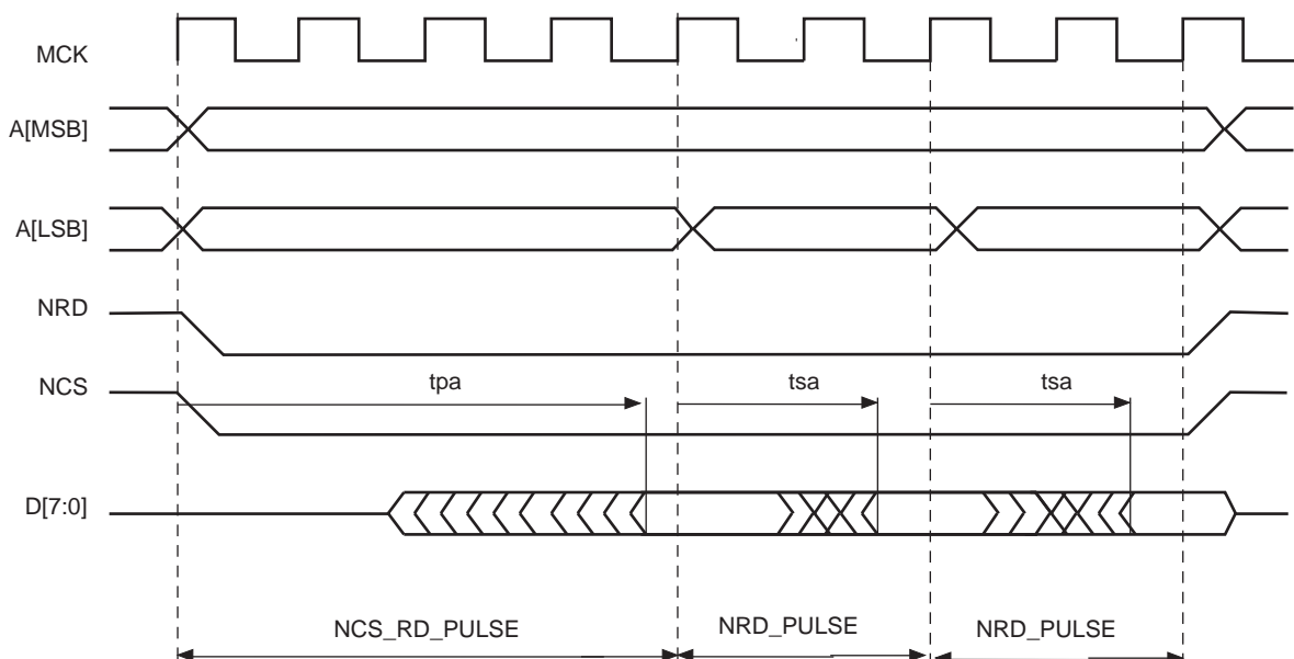
Figure 24-31. Page Mode Read Protocol (Address MSB and LSB are defined in Table 24-5 )
