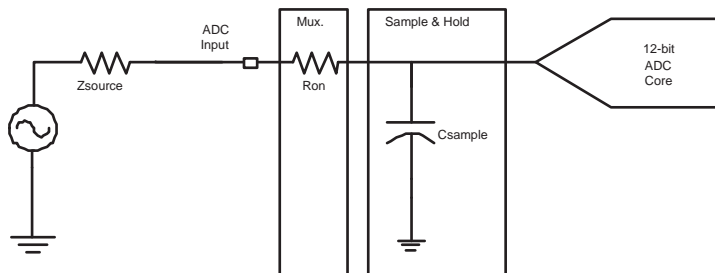
Figure 42-12.Simplified Acquisition Path
