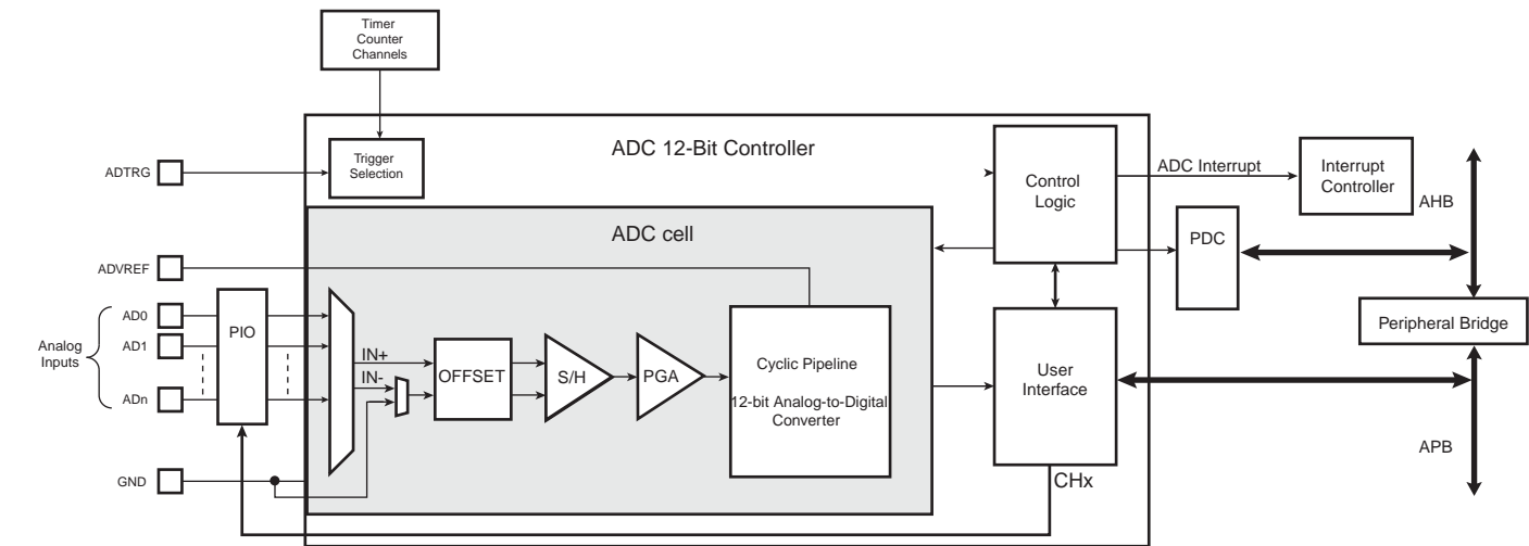
Figure 40-1. Analog-to-Digital Converter Block Diagram
