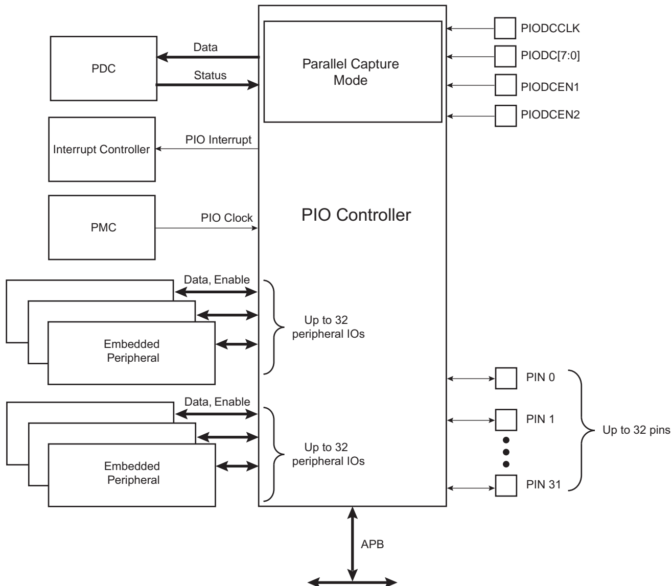
Figure 29-1. Block Diagram
