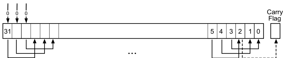
Figure 11-5. LSR #3
