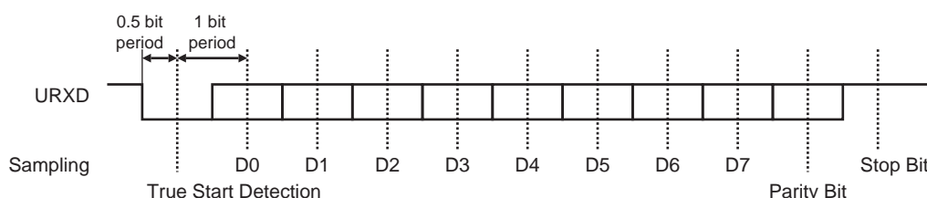
Figure 33-4. Character Reception
