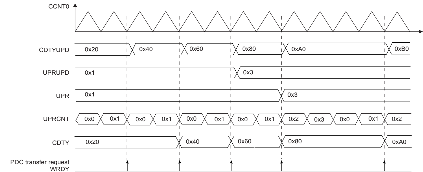
Figure 37-12. Method 3 (UPDM=2 and PTRM=0)
