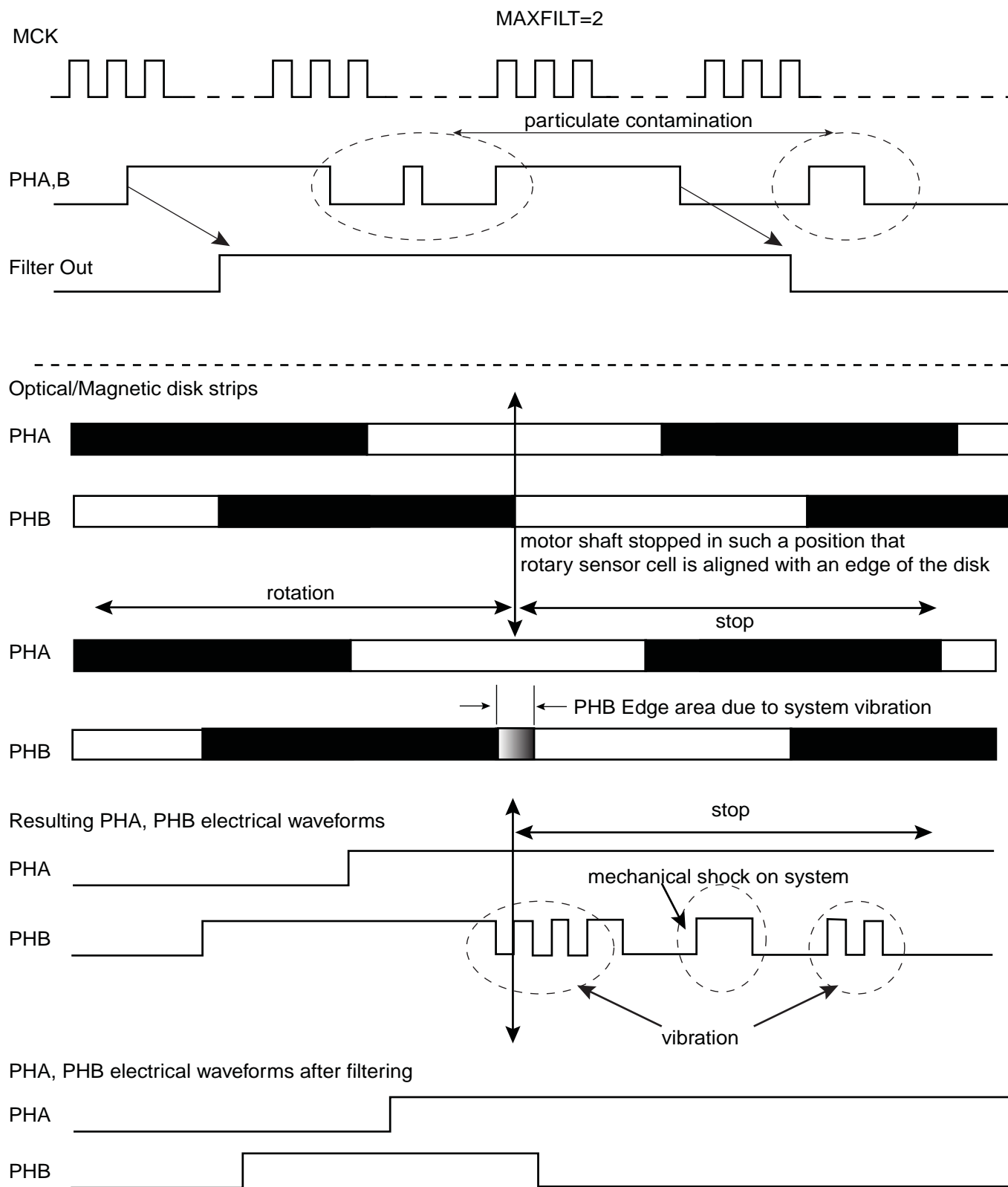
Figure 35-17. Filtering Examples
