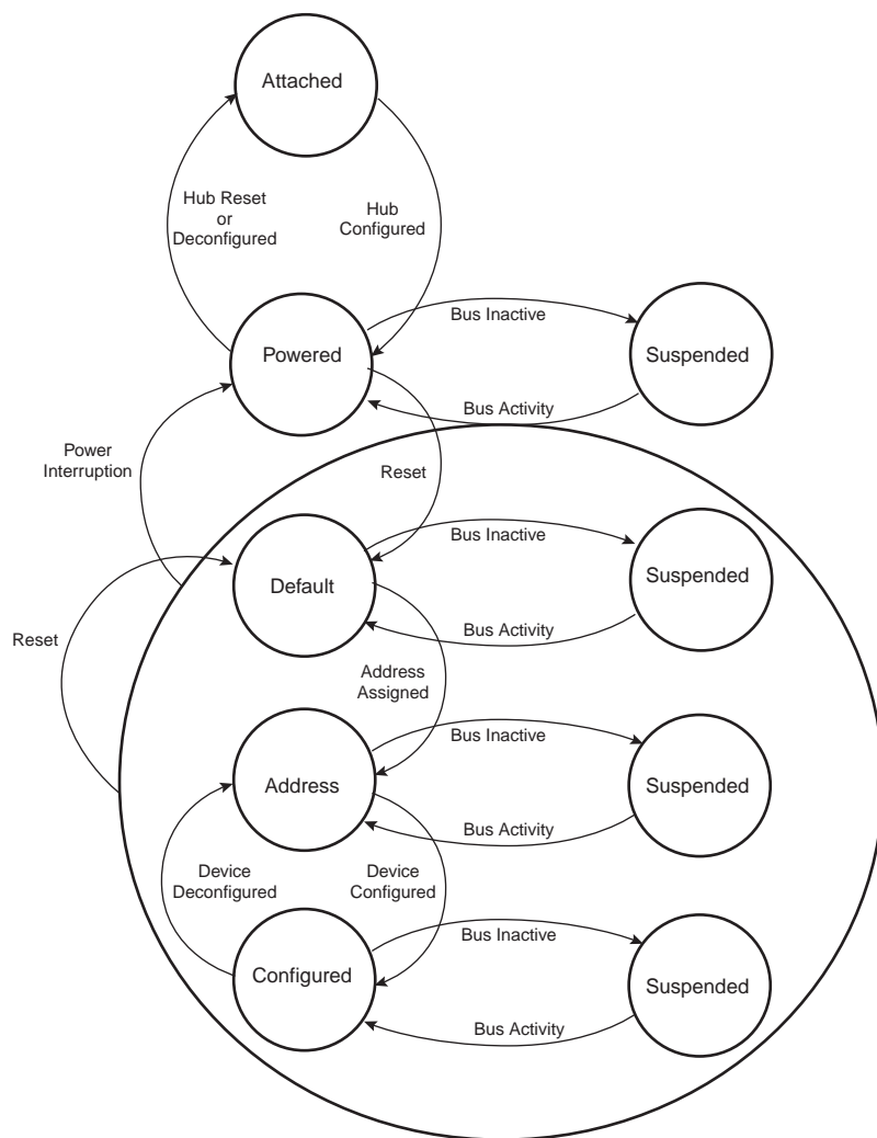
Figure 38-14. USB Device State Diagram
