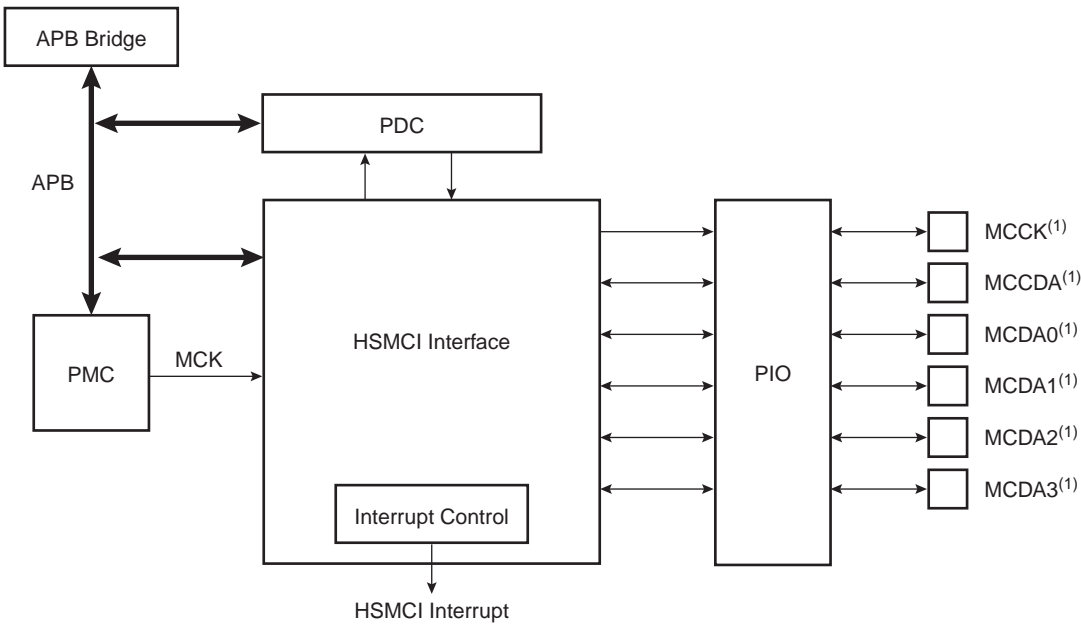
Figure 36-1. Block Diagram
