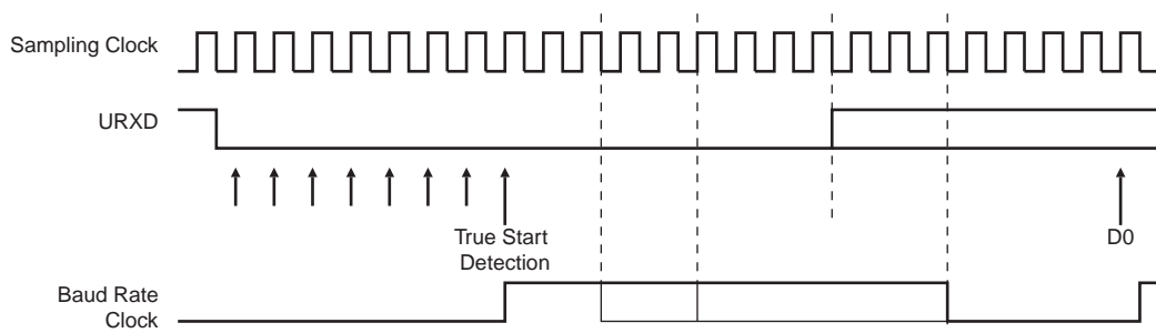
Figure 33-4. Character Reception
