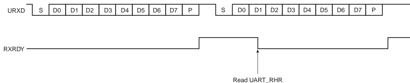
Figure 33-5. Receiver Ready
