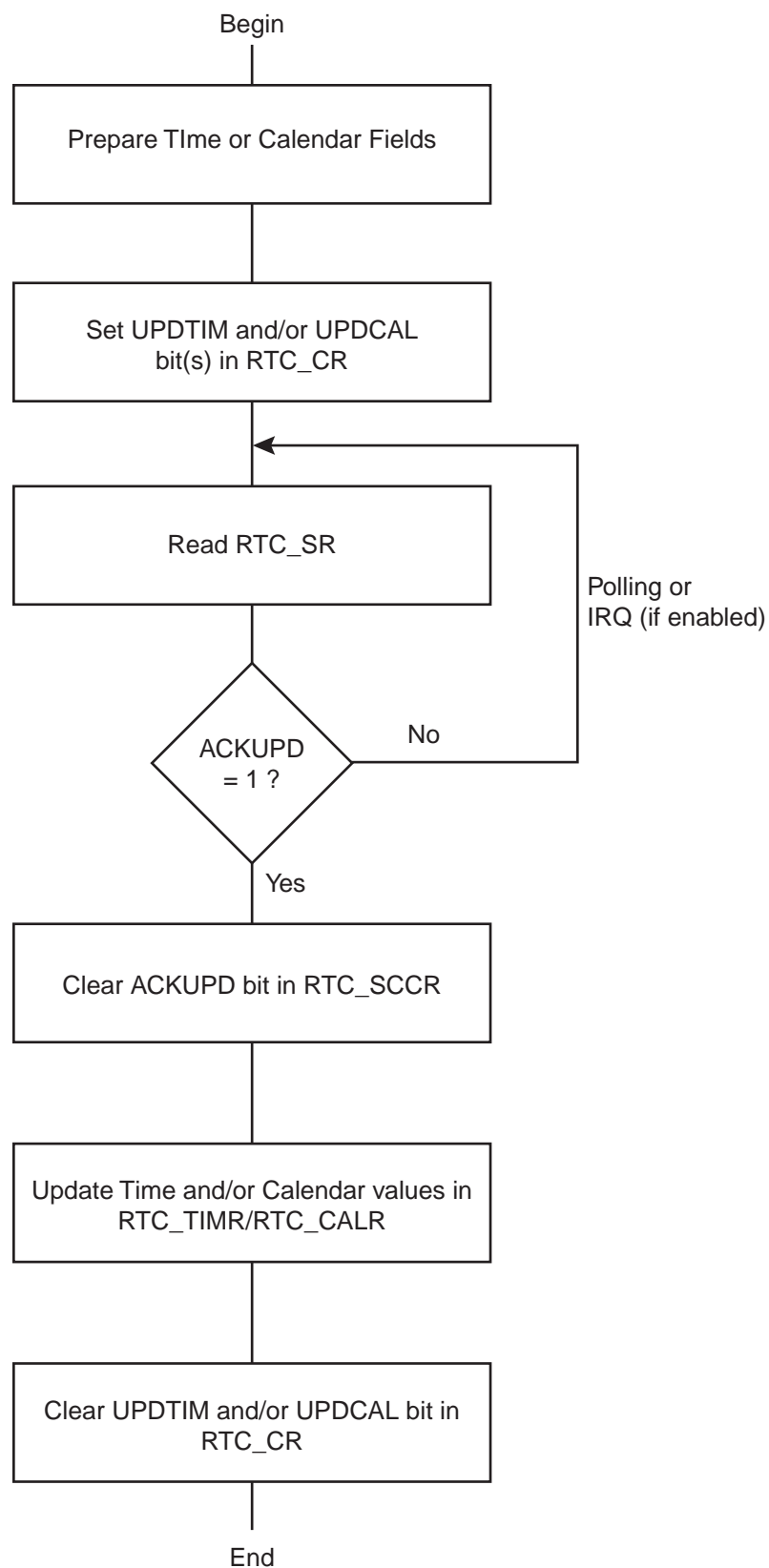
Figure 15-2. Update Sequence
