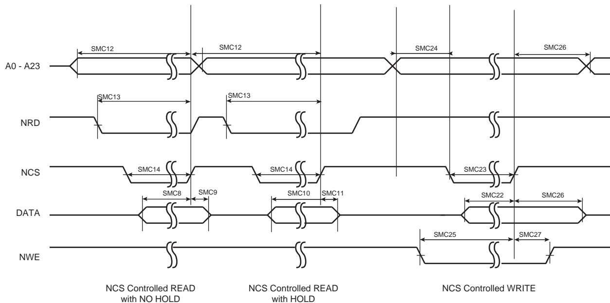
Figure 42-26.SMC Timings - NCS Controlled Read and Write
