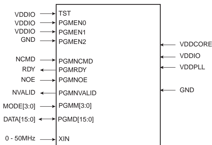
Figure 20-1. SAM3SxA (48 bits) Parallel Programming Interface
