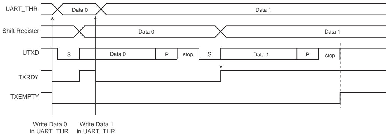
Figure 33-10. Transmitter Control
