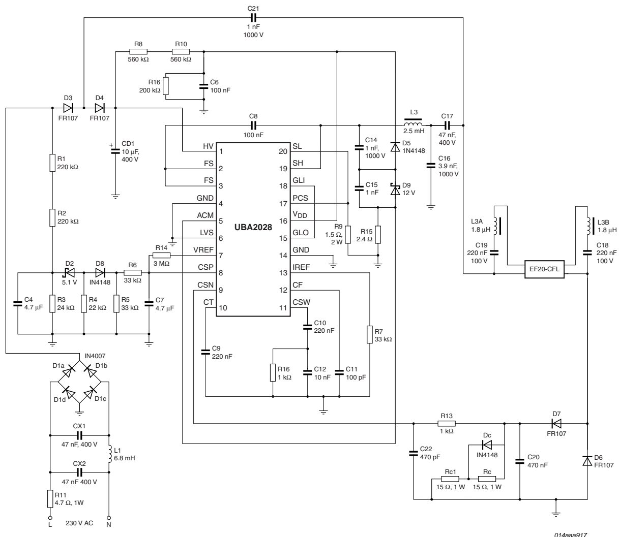
Fig 9. Application circuit 230 V
