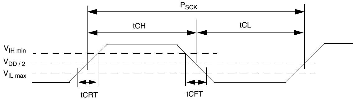
Figure 5.10 Clock Timing
