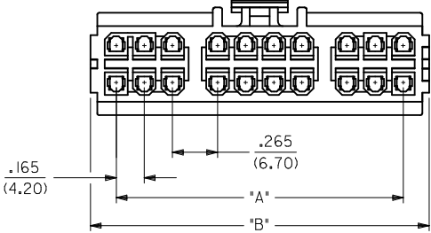
20 CIRCUIT
