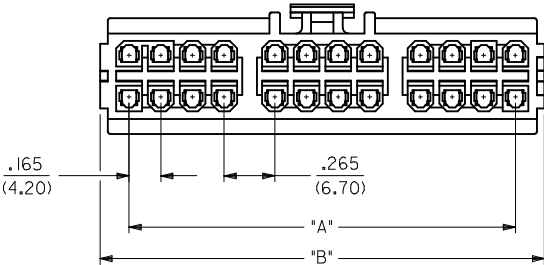
24 CIRCUIT
