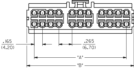
22 CIRCUIT
