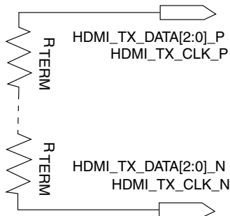
Figure 58. Source Termination
