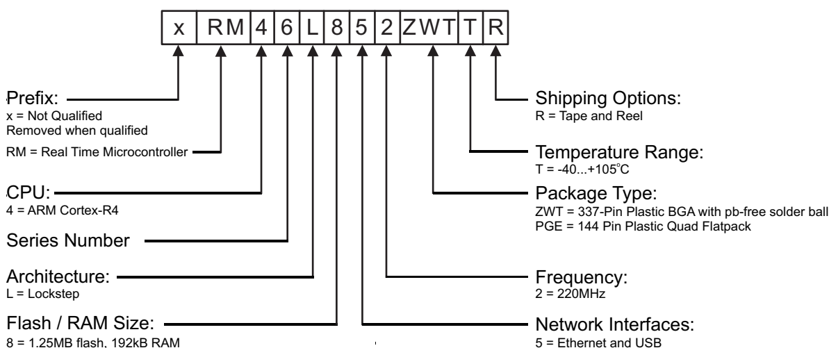
Figure 6-1. RM46L852 Device Numbering Conventions
