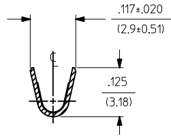
SECT. "B-B"
