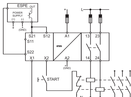
NLG02D - One 2-wire PNP output - Safety cat. 2
