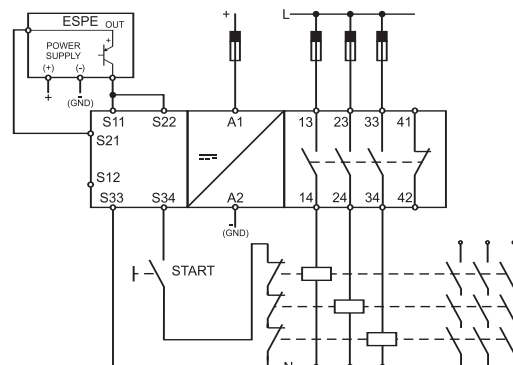
NLG13D - One 2-wire relay output - Safety cat. 2
