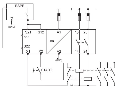
NLG02D - One 2-wire relay output - Safety cat. 2
