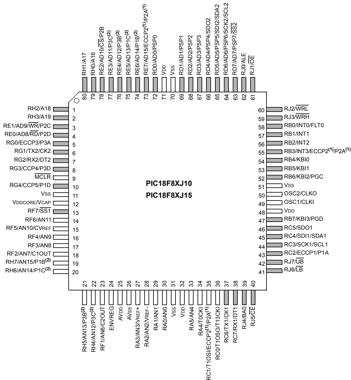
80-Pin TQFP
