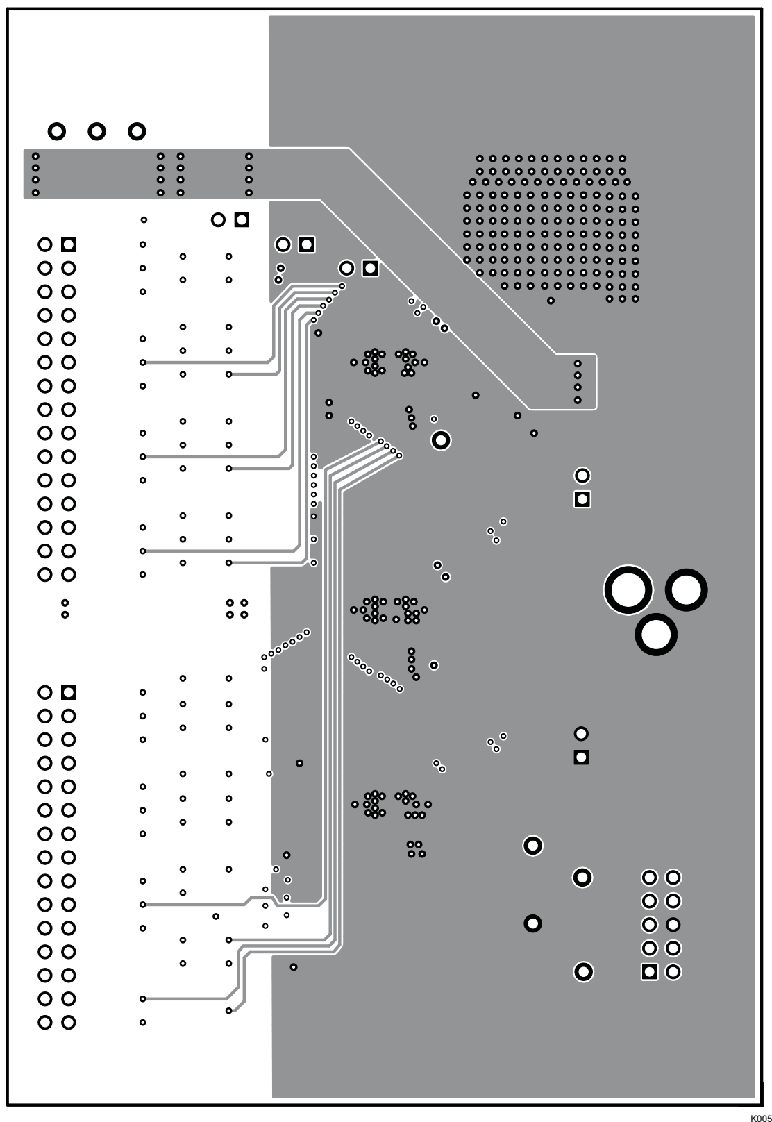
Figure 9. TLC59116FEVM-571 Bottom Layer Routing
