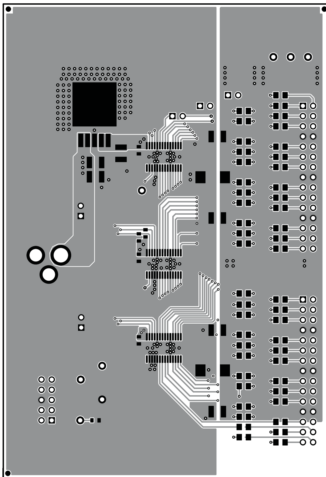
Figure 6. TLC59116FEVM-571 Top Layer Routing
