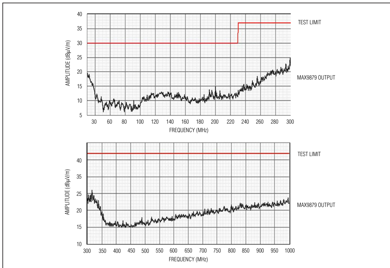
Figure 4. EMI with 152mm of Speaker Cable
