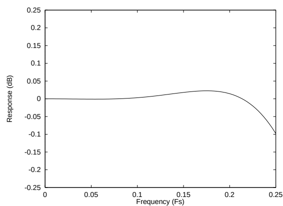
Figure 42 ADC Digital Filter Ripple – Type 3
