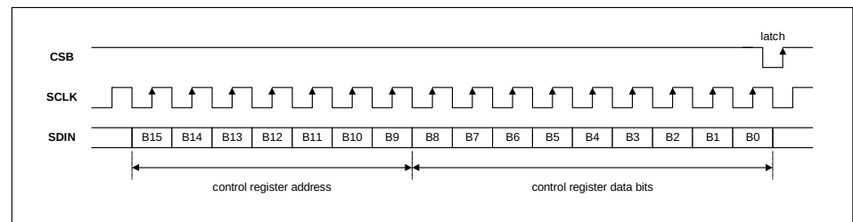
Figure 25 3-Wire Serial Control Interface
