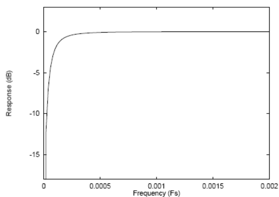
Figure 49 ADC Highpass Filter Response
