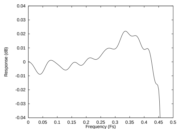
Figure 36 ADC Digital Filter Ripple – Type 0
