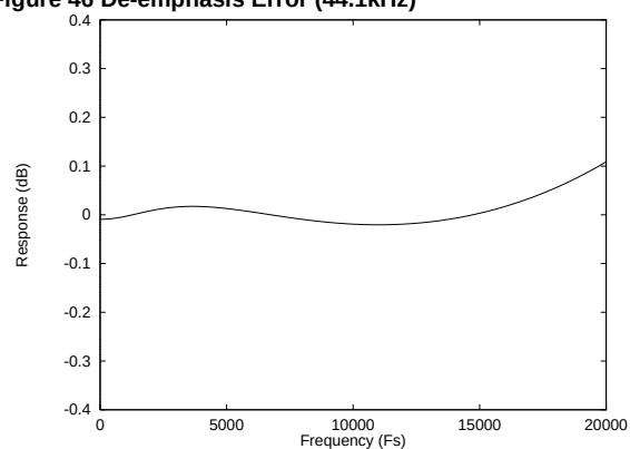
Figure 48 De-emphasis Error (48kHz)
