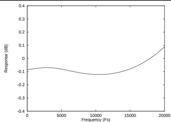
Figure 46 De-emphasis Error (44.1kHz)
