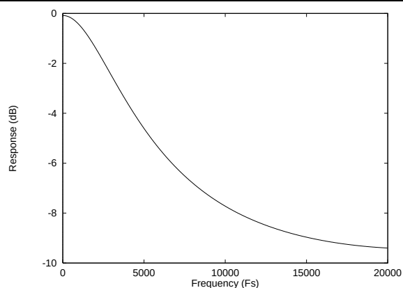
Figure 45 De-emphasis Frequency Response (44.1kHz)
