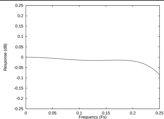
Figure 40 ADC Digital Filter Ripple – Type 2
