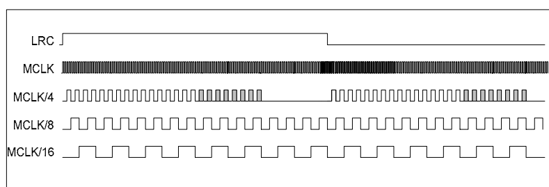
Figure 24 Bit Clock Mode
