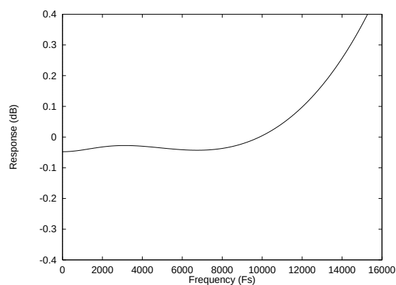
Figure 44 De-emphasis Error (32kHz)
