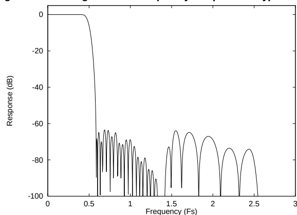
Figure 37 ADC Digital Filter Frequency Response – Type 1
