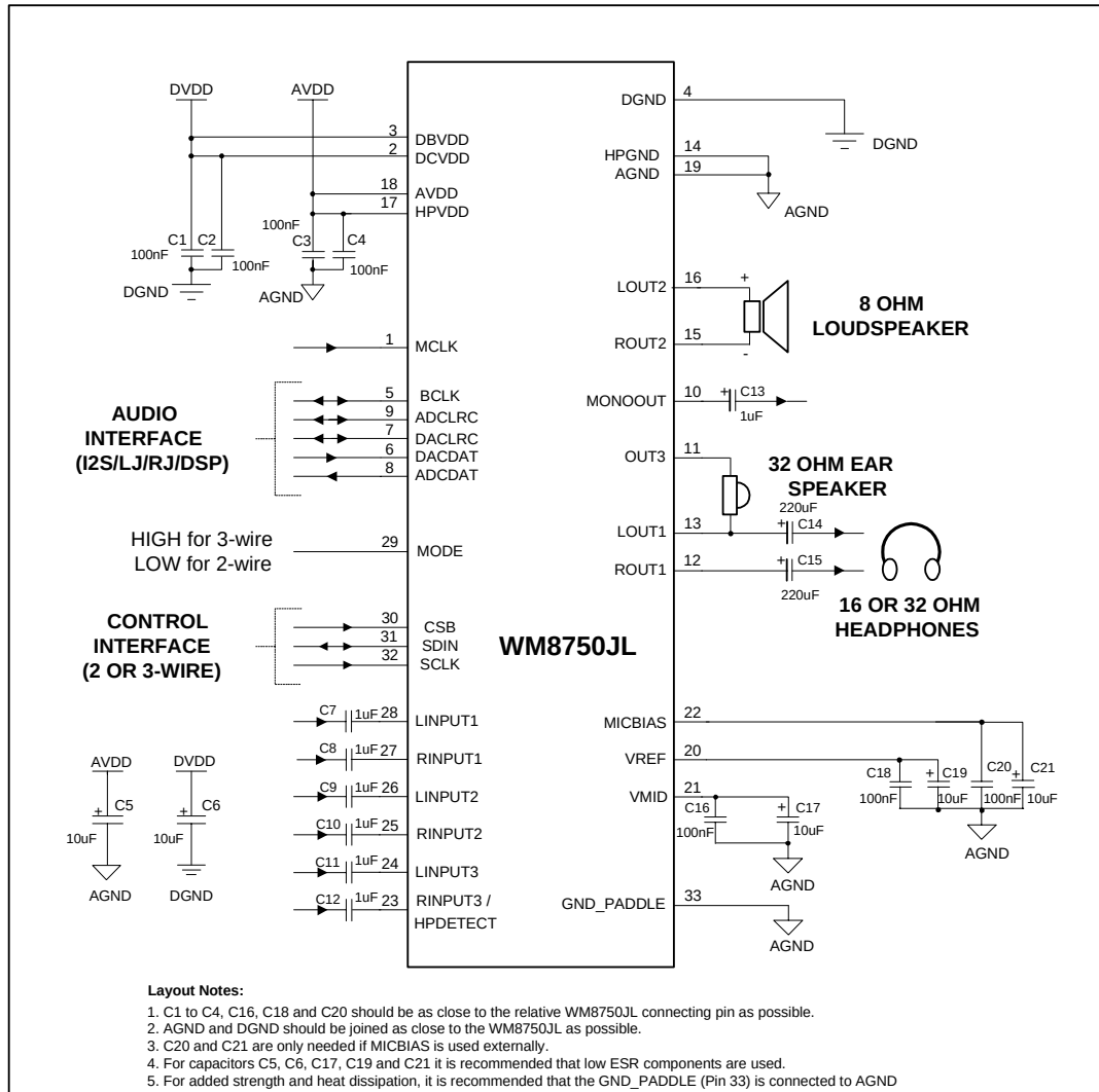
Figure 50 Recommended External Components Diagram
