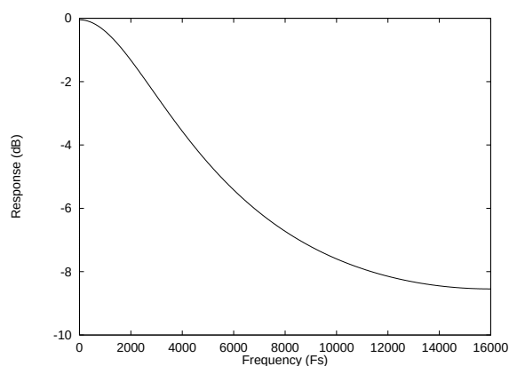
Figure 43 De-emphasis Frequency Response (32kHz)
