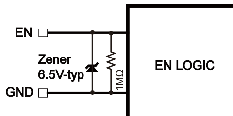
Figure 2: 6.5V Zener Diode
