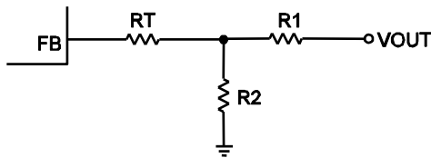
Figure 4: T-Type Network
