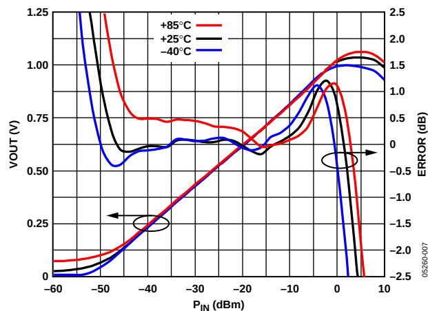
Figure 7. VOUT and Log Conformance vs. Input Amplitude at 2.2 GHz; Typical Device at -40^\circ\text{C} , +25^\circ\text{C} , and +85^\circ\text{C}
