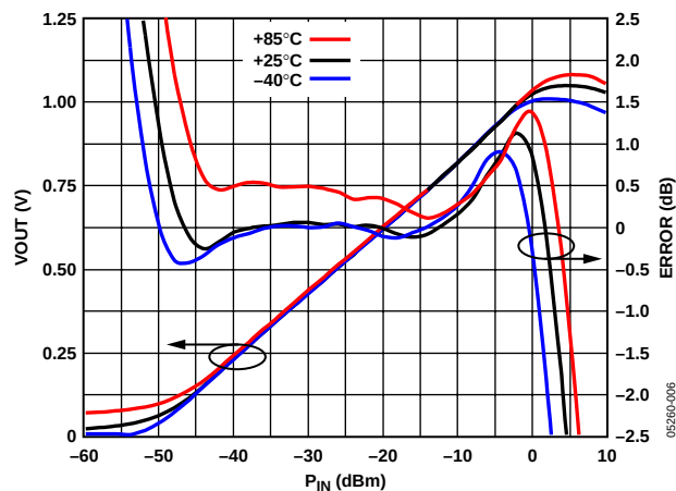
Figure 6. VOUT and Log Conformance vs. Input Amplitude at 1.9 GHz; Typical Device at -40^\circ\text{C} , +25^\circ\text{C} , and +85^\circ\text{C}
