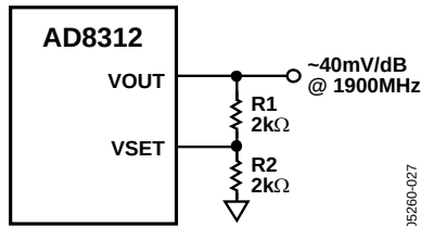
Figure 27. Increasing the Output Slope
