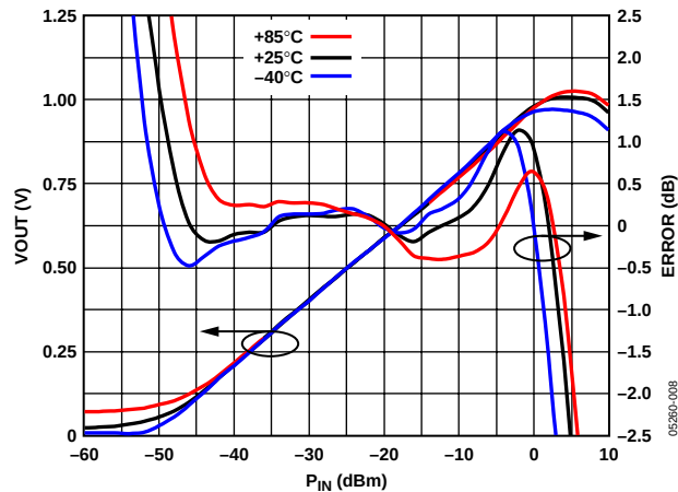
Figure 8. VOUT and Log Conformance vs. Input Amplitude at 2.5 GHz; Typical Device at -40^\circ\text{C} , +25^\circ\text{C} , and +85^\circ\text{C}
