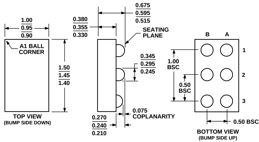
Figure 38. 6-Ball Wafer-Level Chip Scale Package [WLCSP] (CB-6)
