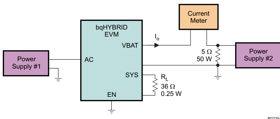
Figure 2-4. Test Setup C
