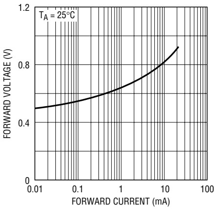
Foward Characteristics
