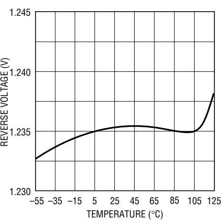
Temperature Drift
