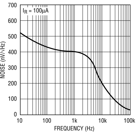
Noise Voltage
