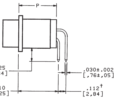
Termination Style 6
