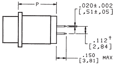
Termination Style 2
