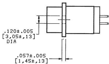
Mounting Style 1
