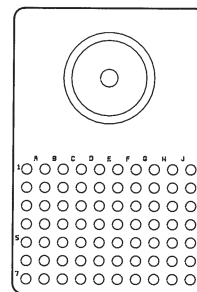
Insert 71C1A 70 #22 Contacts 1 #1 Coax Contact
