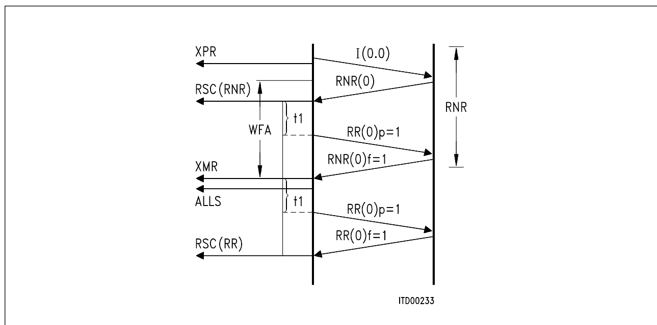
Figure 24 Flow Control/Transmission
