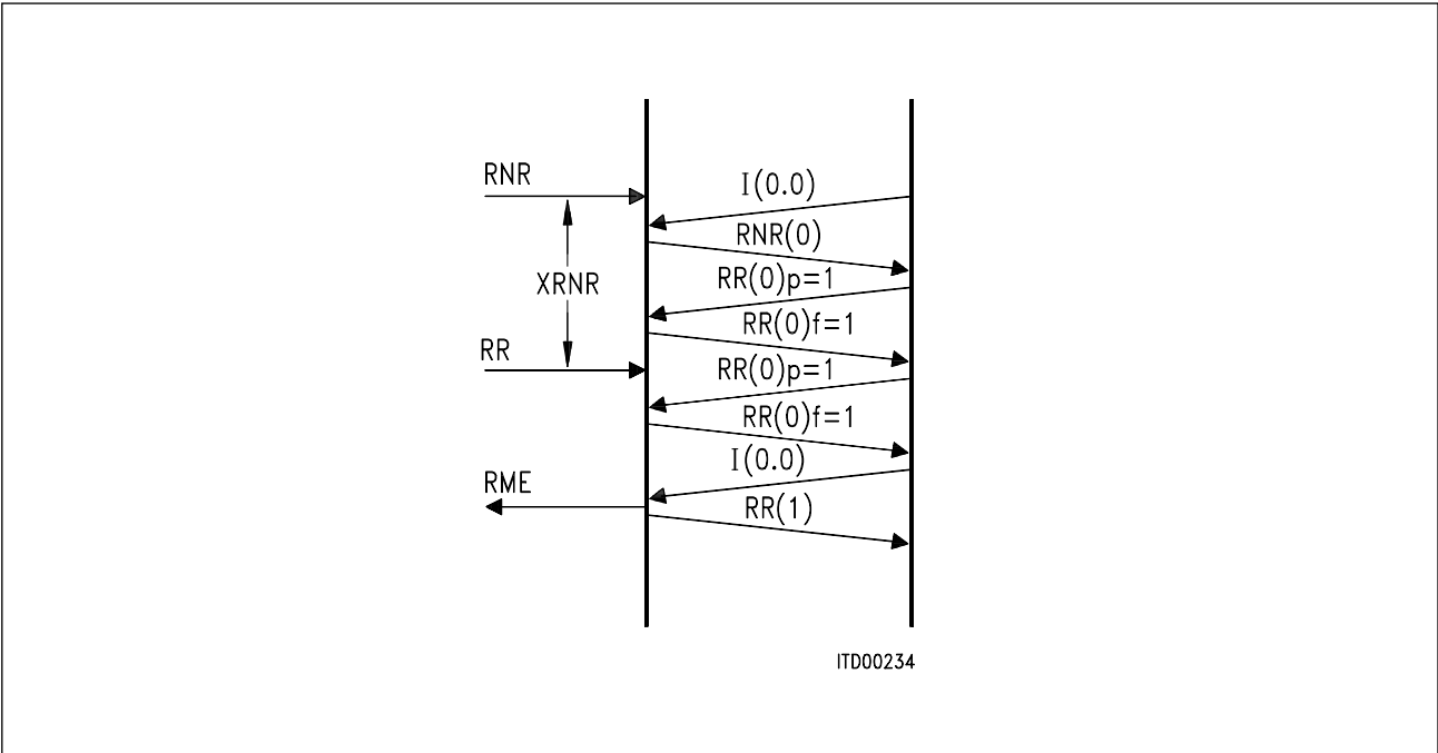
Figure 25 Flow Control/Reception
