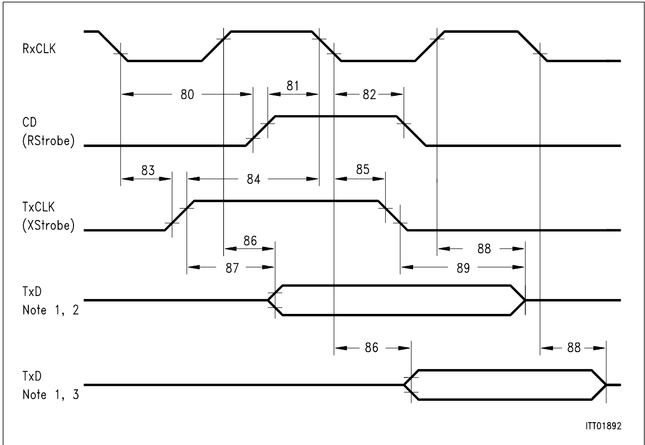
Figure 69 Strobe Timing
