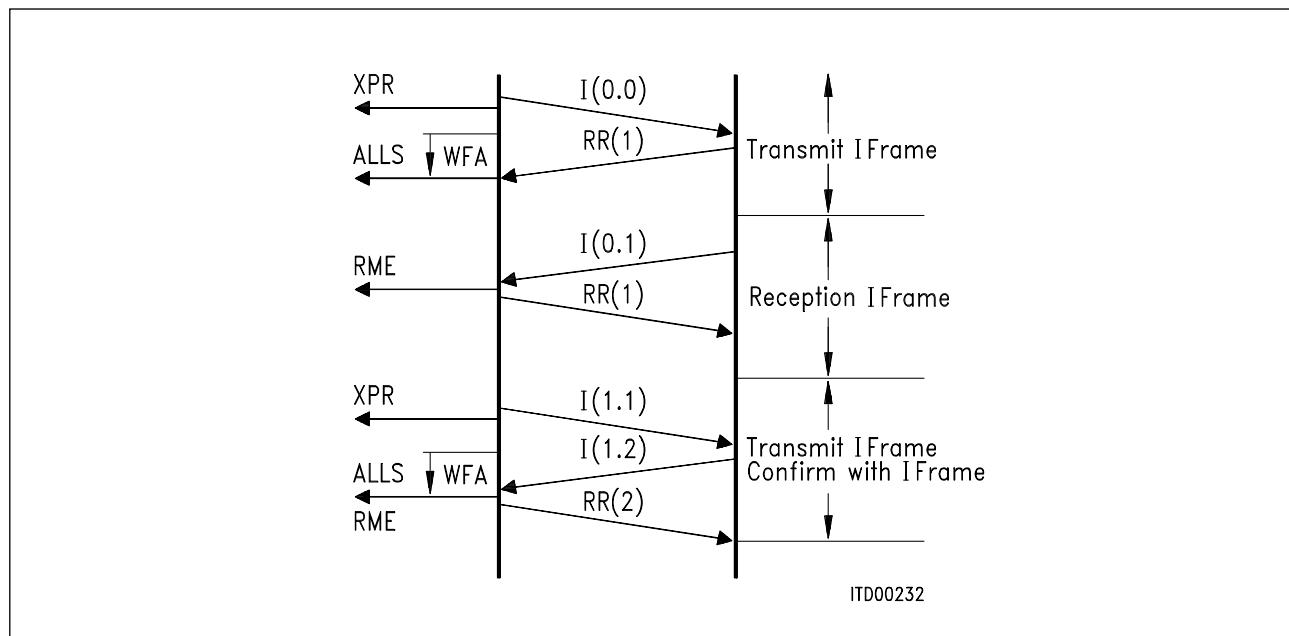
Figure 23 Transmission/Reception I-Frames
