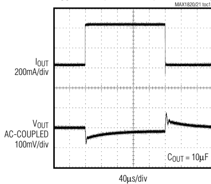
LOAD TRANSIENT ( I_{LOAD} = 20\text{mA} TO 420\text{mA} , V_{OUT} = 1.5\text{V} , V_{IN} = 3.6\text{V} , SKIP = BATT )
