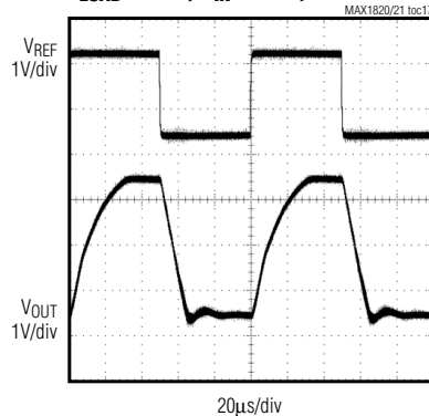
REF TRANSIENT ( V_{REF} = 0.23\text{V} TO 1.932\text{V} , R_{LOAD} = 10\Omega , V_{IN} = 3.6\text{V} , SKIP = BATT )
