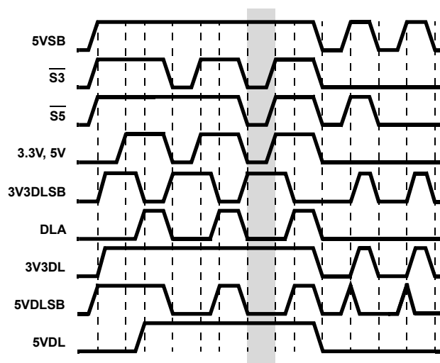
FIGURE 5. 5V_{DUAL} AND 3.3V_{DUAL}/3.3V_{SB} TIMING DIAGRAM; ISL6504A
