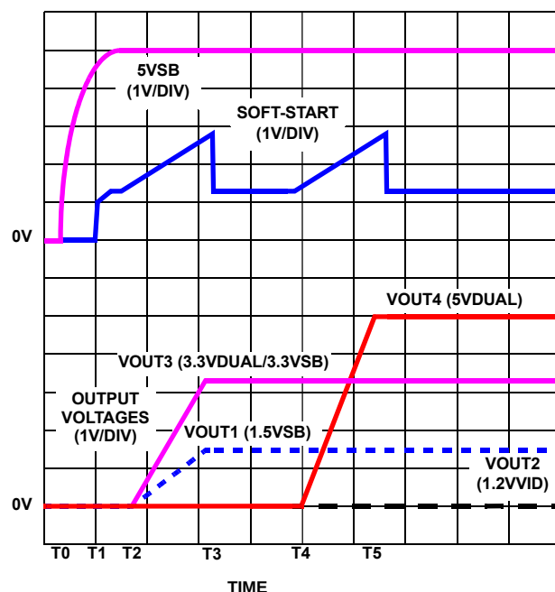
FIGURE 8. SOFT-START INTERVAL IN A SLEEP STATE; ISL6504A
