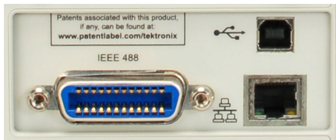
PA1000 rear panel communication ports
