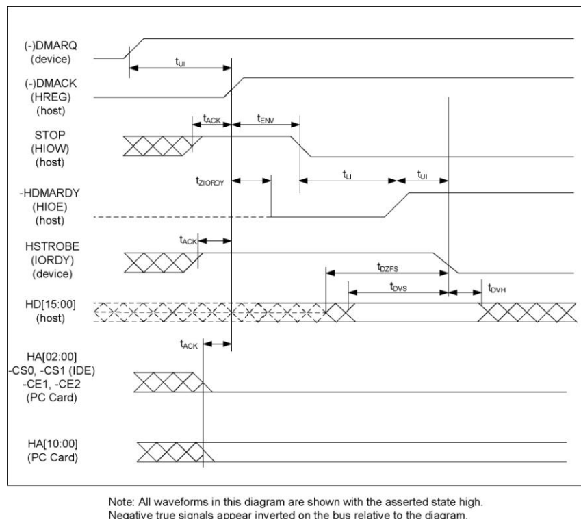
Figure 17: UDMA Data-Out Burst Initiation Timing
