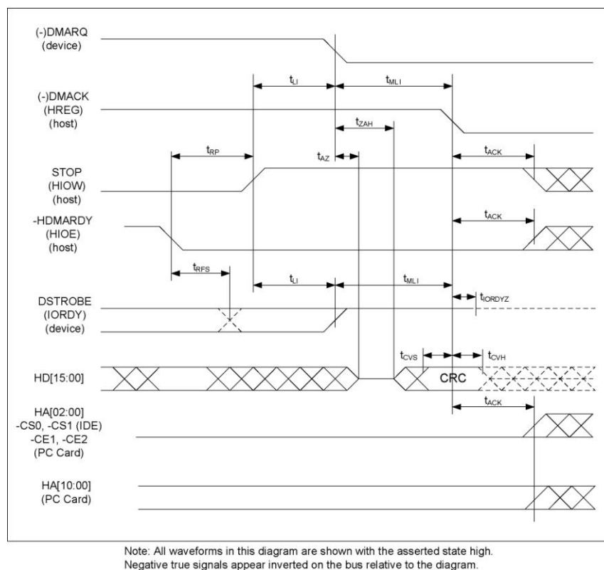
Figure 16: UDMA Data-In Burst Host Termination Timing
