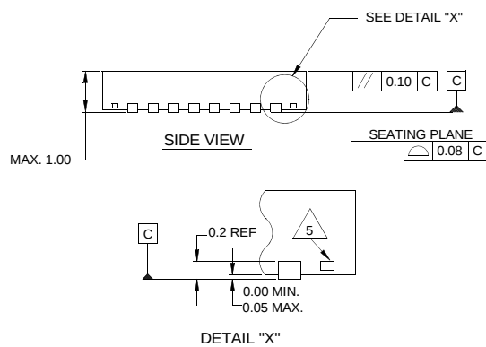
DETAIL "X"
