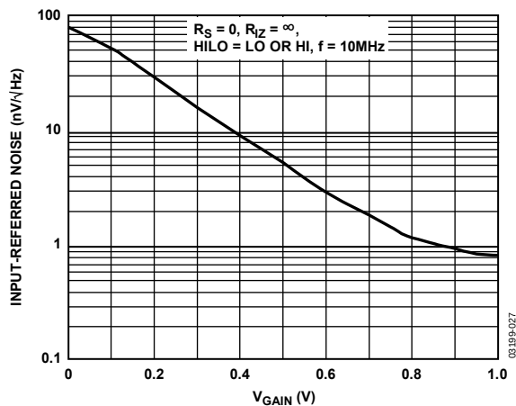
Figure 27. Short-Circuit, Input-Referred Noise vs. V_{\text{GAIN}}
