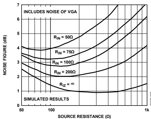
Figure 30. Noise Figure vs. R_S for Various Values of R_{\text{IN}}
