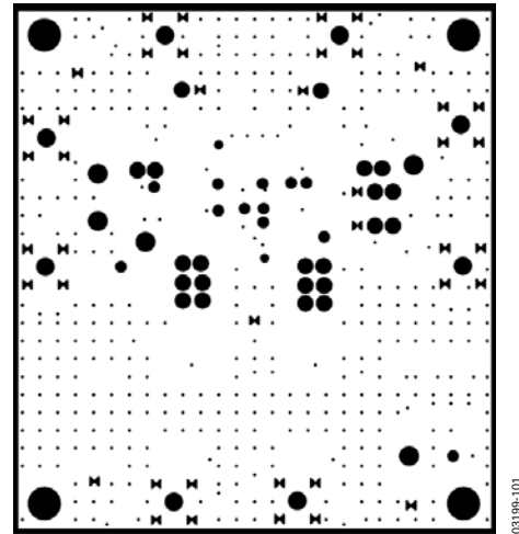
Figure 110. Ground Plane
