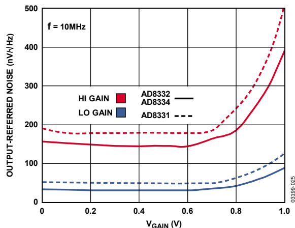
Figure 25. Output-Referred Noise vs. V_{\text{GAIN}}
