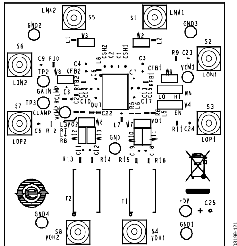
Figure 107. AD8332-EVALZ Assembly
