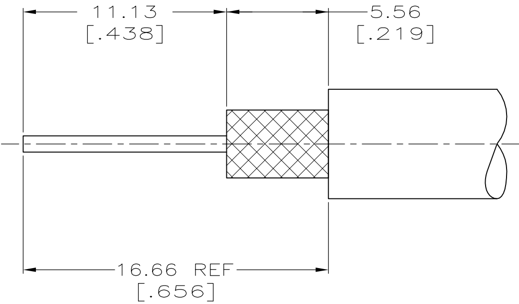
RECOMMENDED STRIP LENGTH NO SCALE
