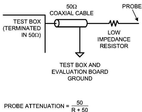
FIGURE 3. Probe Schematic
