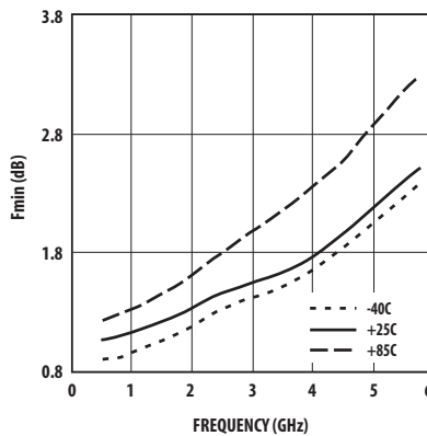
Figure 6. Fmin vs. Frequency and Temperature.
