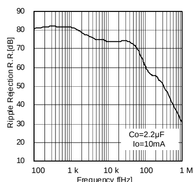
Fig.18 Ripple Rejection (BH33NB1WHFV)
