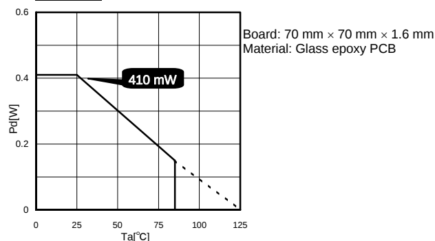
Fig. 26 HVSO5F5 Power Dissipation/Power Dissipation Reduction (Example)
