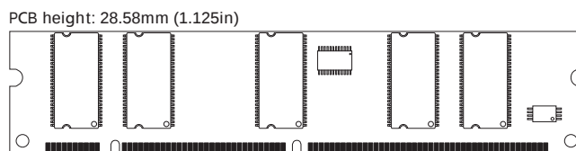
Figure 2: Low Profile Layout
