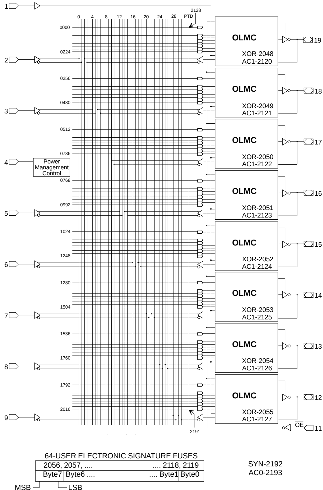
PLCC Package Pinout
