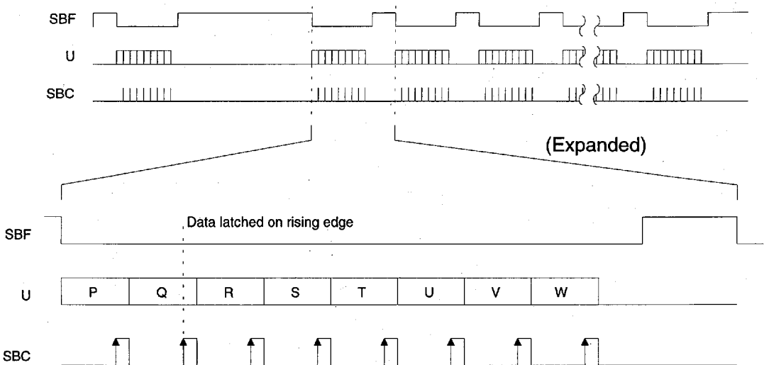
Figure 22. CD Subcode Port Timing
