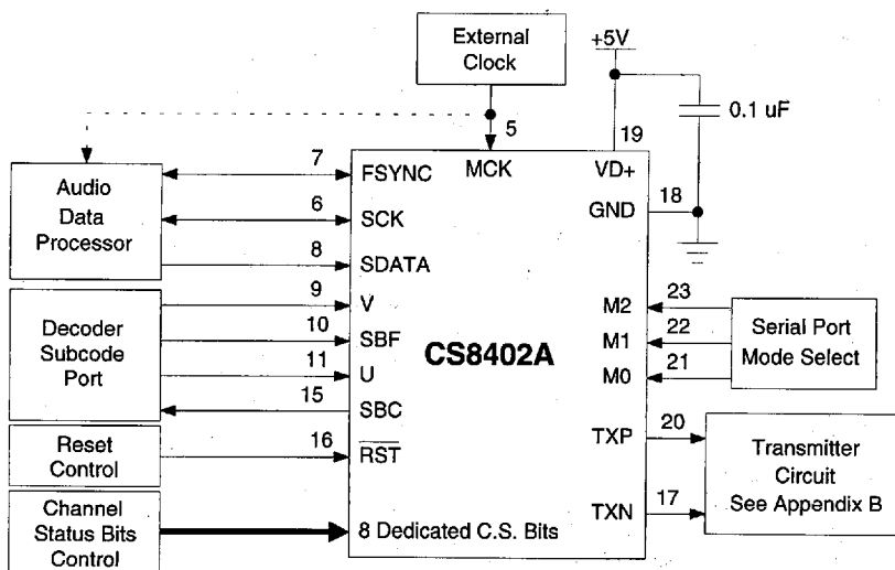
Figure 3. Consumer CD Submode Typical Connection Diagram
