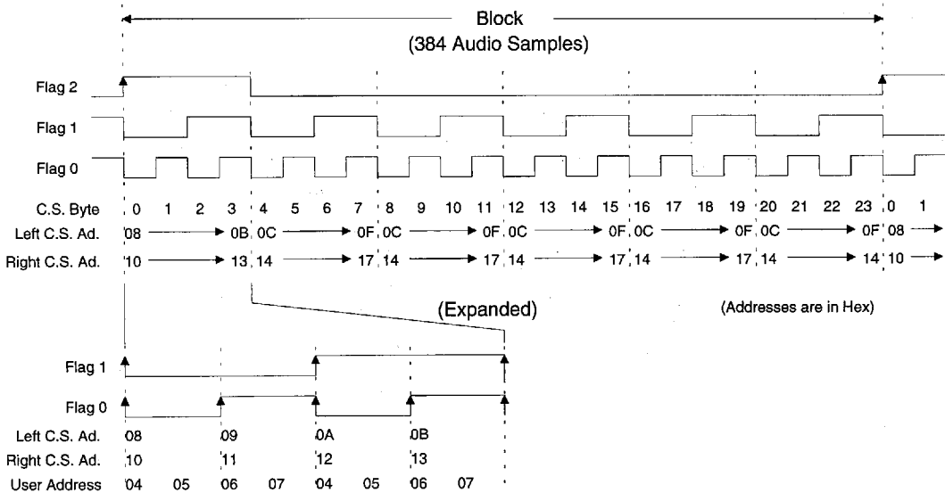
Figure 14. CS8401A Buffer Memory Read Sequence - MODE 2
