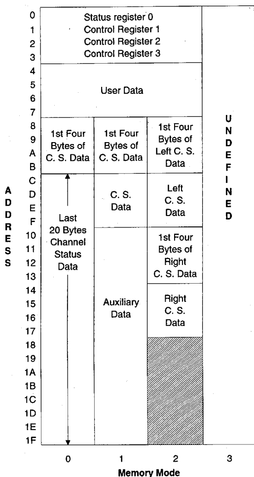
Figure 5. CS8401A Buffer Memory Modes
