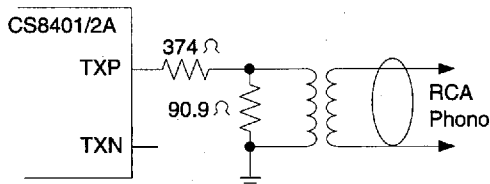
Figure A2. Consumer Output Circuit
