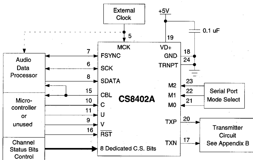
Figure 2. CS8402A Professional & Consumer Modes Typical Connection Diagram
