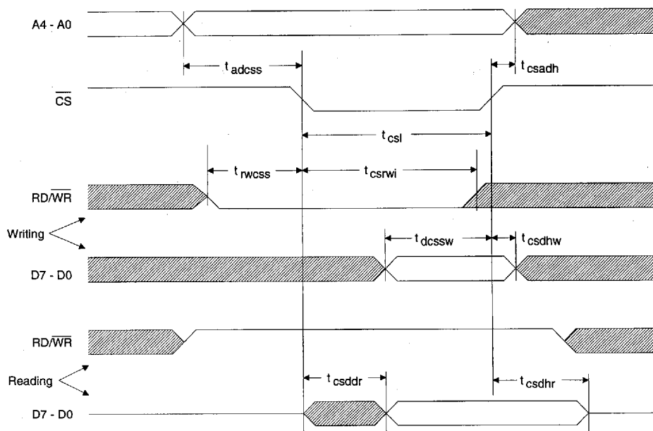
CS8401A Parallel Port Timing
