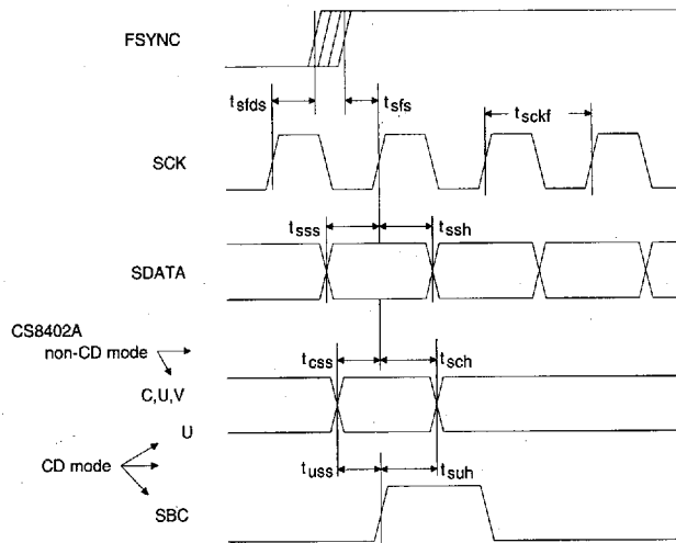
Serial Input Timing - Master Mode & C, U, V Port
