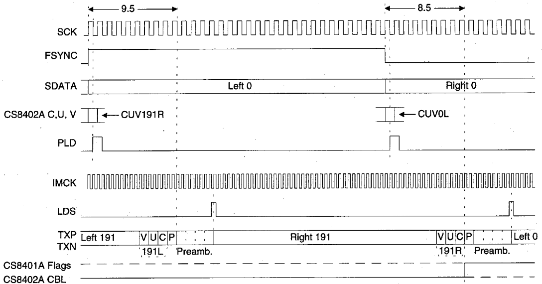
Figure B2. Serial Ports-to-Transmitter Timing (slave mode)
