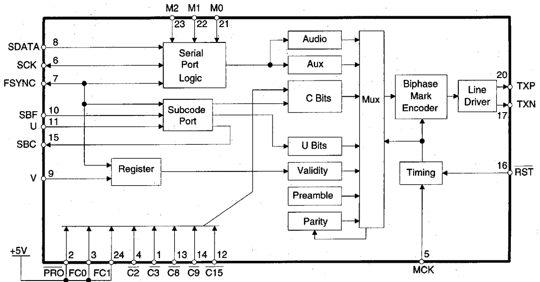
Figure 21. CS8402A Block Diagram - Consumer Mode, CD Submode
