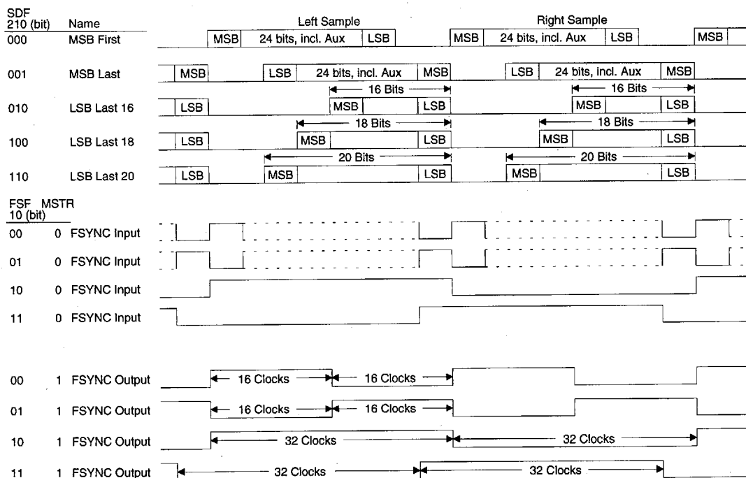
Figure 10. CS8401A Serial Port SDATA and FSYNC Timing
