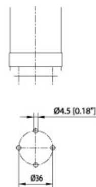
Direct Mounting
