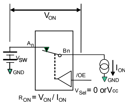
Figure 3. On Resistance
