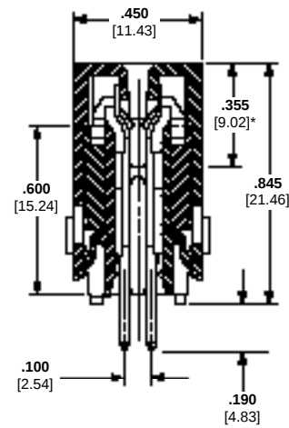
Section P-P
