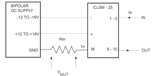
Connection Schematic
