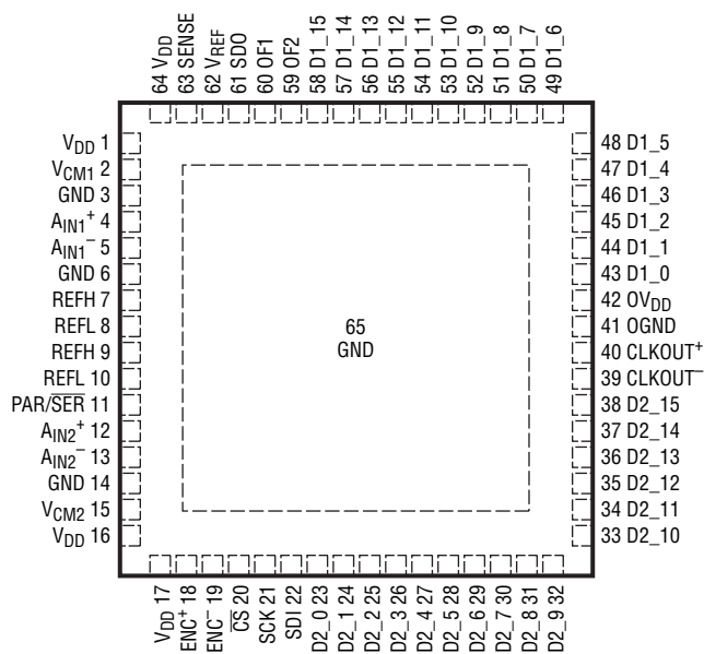
FULL-RATE CMOS OUTPUT MODE
