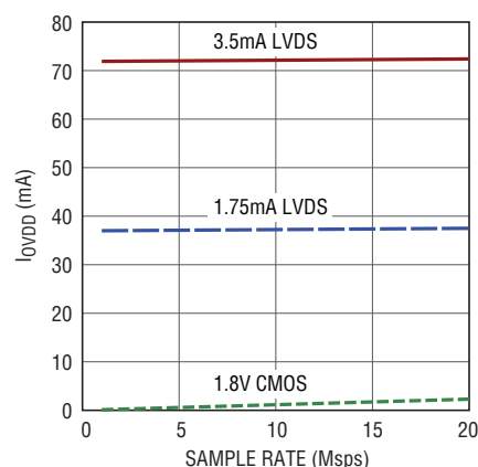
I_{QVDD} vs Sample Rate, 5MHz, -1dBFS Sine Wave Input on Each Channel
