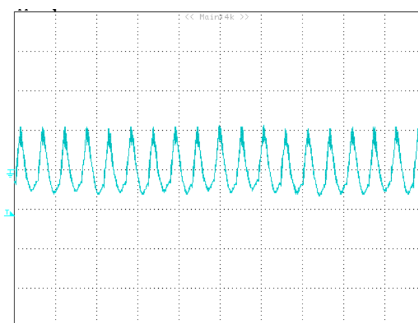
Figure 9: Output ripple & noise at 11.0V in , 1.0V/ 80A out 20mV/div, 2uS/div
