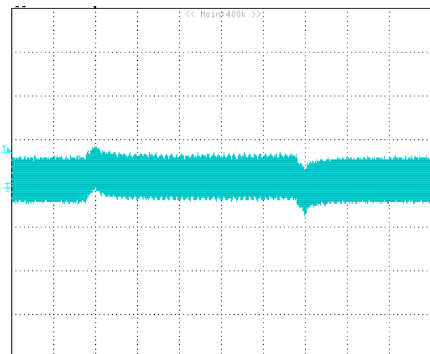
Figure 18: Typical transient response, 11.0Vin/1.8Vo 50mV/div, 200uS/div (Load Step: 50% ~ 100%~50% Iout, slew rate=0.5A/uS)
