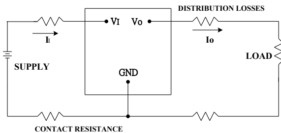
Figure 22: Output voltage and efficiency measurement test setup
