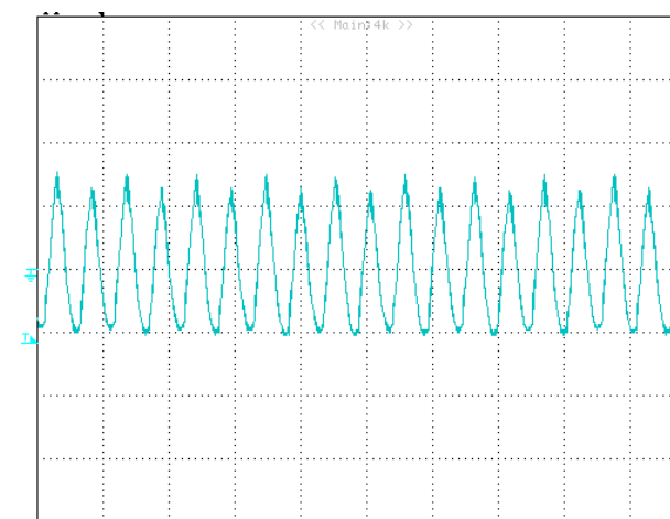
Figure 11: Output ripple & noise at 11.0V in , 1.8V/ 80A out 20mV/div, 2uS/div
