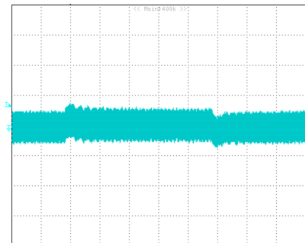
Figure 20: Typical transient response, 11.0Vin/3.3Vo 50mV/div, 200uS/div (Load Step: 50% ~ 100%~50% Iout, slew rate=0.5A/uS)
