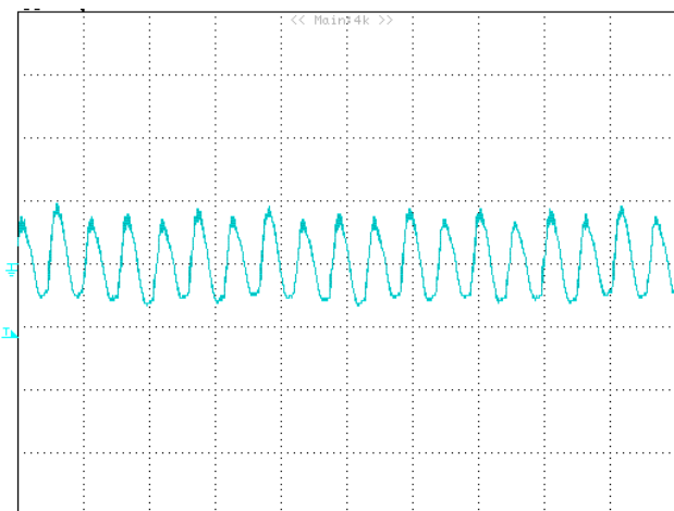
Figure 8: Output ripple & noise at 11.0V in , 1.0V/ 0A out 20mV/div, 2uS/div
