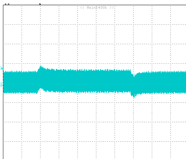
Figure 19: Typical transient response, 11.0Vin/2.5Vo 50mV/div, 200uS/div (Load Step: 50% ~ 100%~50% Iout, slew rate=0.5A/uS)
