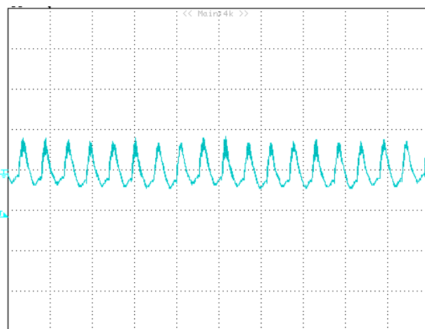
Figure 7: Output ripple & noise at 11.0V in , 0.6V/80A out 20mV/div, 2uS/div
