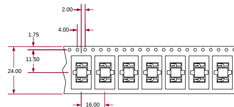
LS Tape & Reel Packaging
