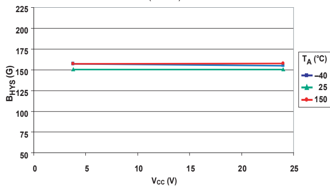
Hysteresis versus Supply Voltage (A1210)
