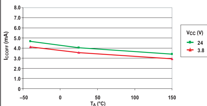
Supply Current (Off) versus Ambient Temperature (A1210/11/12/13/14)
