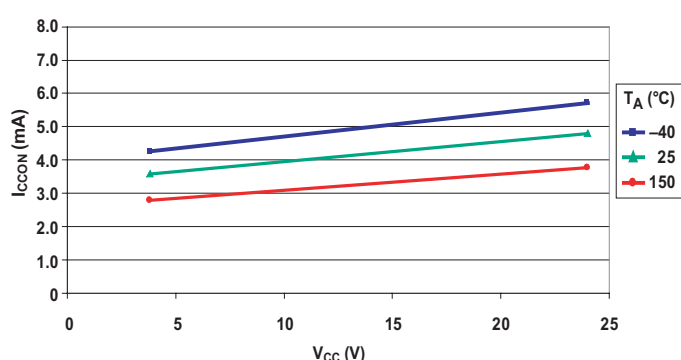
Supply Current (On) versus Supply Voltage (A1210/11/12/13/14)
