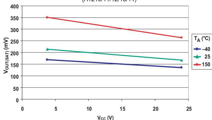
Output Voltage (On) versus Supply Voltage (A1210/11/12/13/14)
