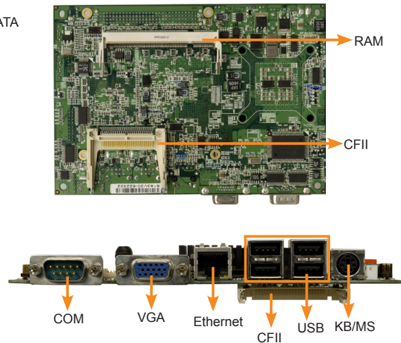
Solder Side
