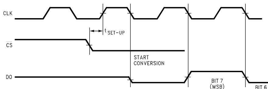
Figure 15. ADC08031 Timing
