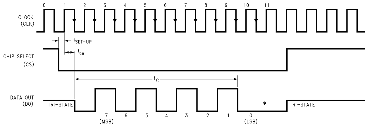
Figure 15. ADC08031 Timing
