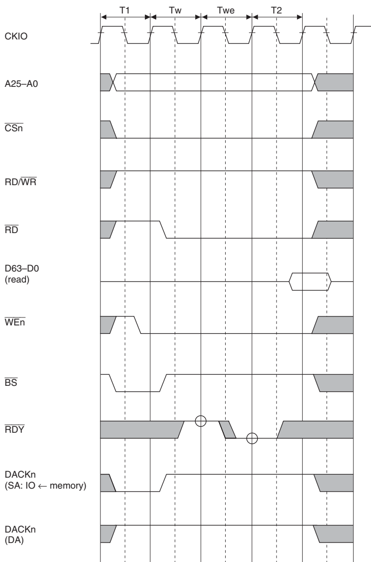
Figure 13.77 Byte Control SRAM Basic Read Cycle (One Internal Wait + One External Wait)
