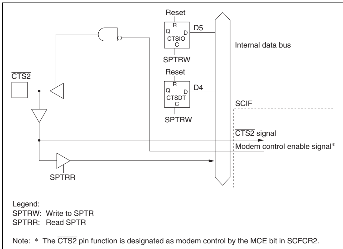
Figure 16.3 \overline{\text{CTS2}} Pin
