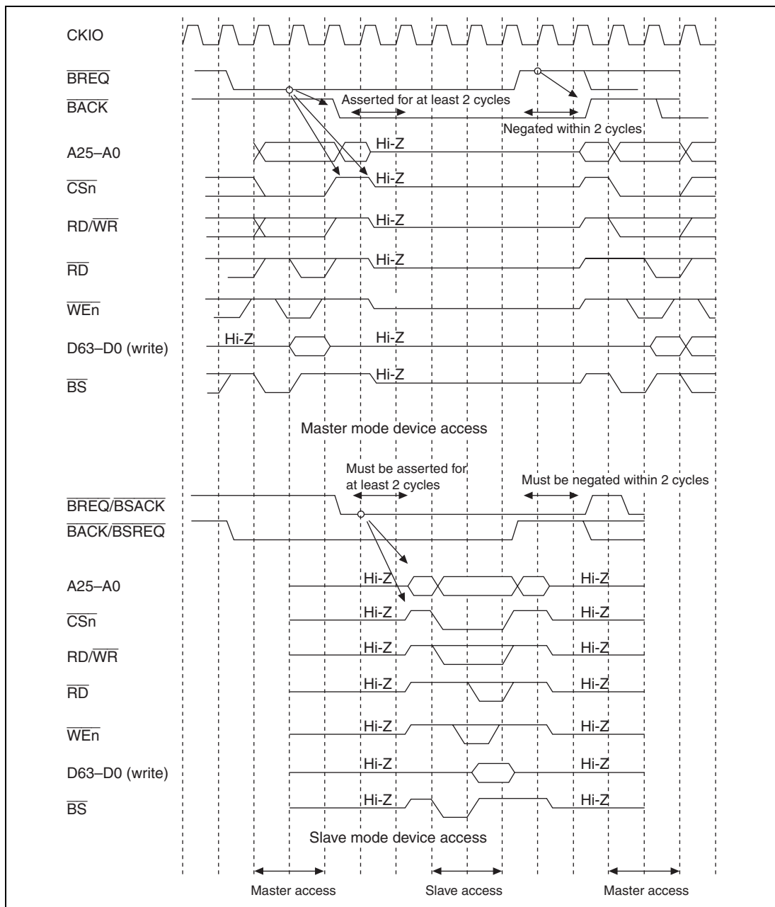
Figure 13.79 Arbitration Sequence
