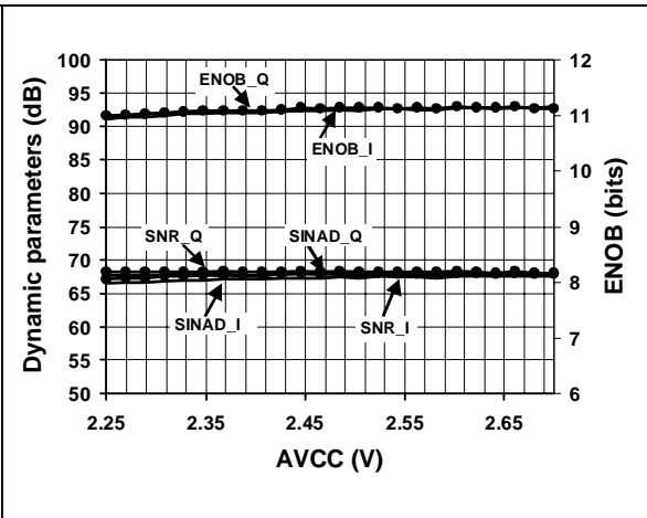
Linearity vs. AVCC F_s=20\text{MSPS} ; I_{cca}=40\text{mA} ; F_{in}=5\text{MHz}
