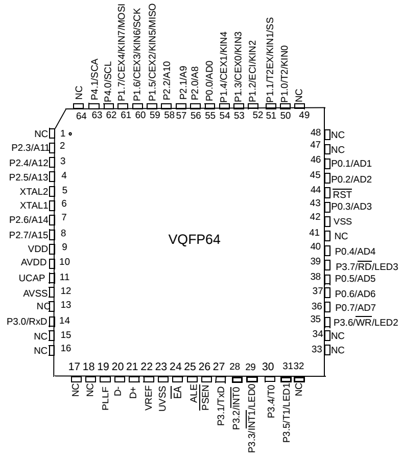
Figure 2. AT89C5131A-M 64-pin VQFP Pinout
