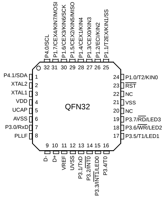
Figure 3. AT89C5131A-M 32-pin QFN Pinout
