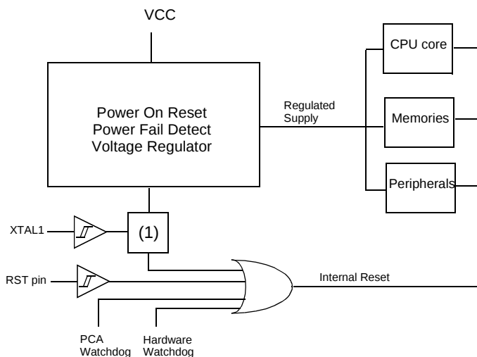
Figure 72. Power Monitor Block Diagram
