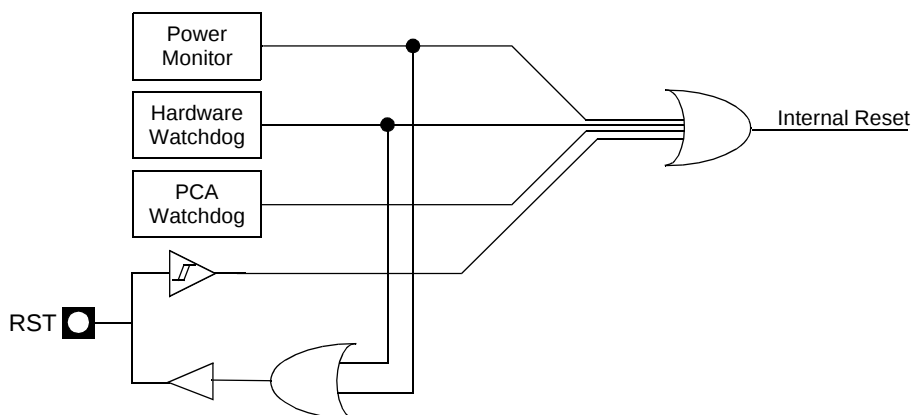
Figure 69. Reset schematic
