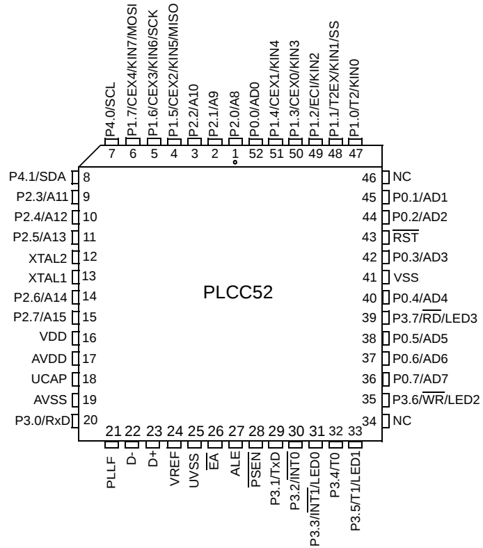
Figure 1. AT89C5131A-M 52-pin PLCC Pinout
