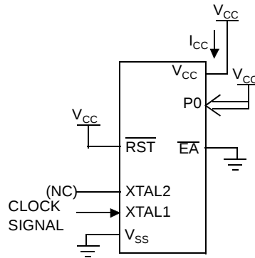
Figure 76. I_{CC} Test Condition, Idle Mode
