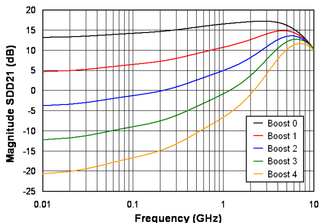
FIGURE 5. GAIN PROFILE FOR VARIOUS BOOST SETTINGS IN QLx411GRx
