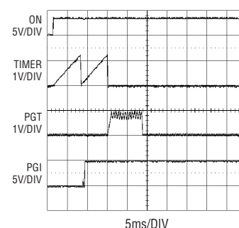
Power-Up Waveforms
